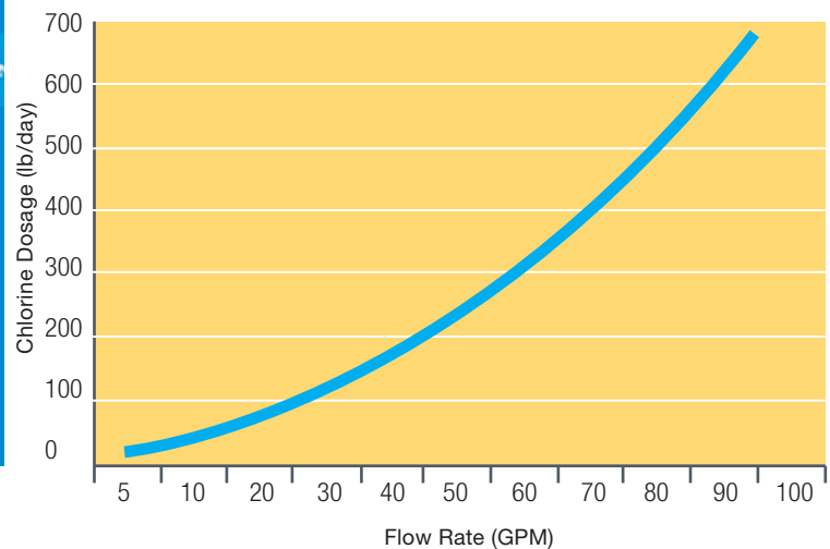
CHLORINATOR DELIVERY RATE MODEL 361000
